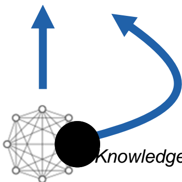
Immunologic Network
